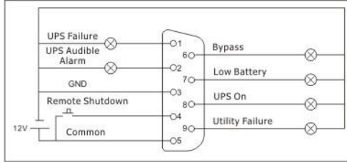
User Interface for 12 V
