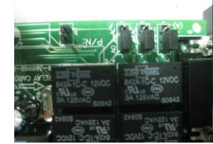
Fig. 5 AO and AC silk printings indicates each 3-pin connector status To achieve ACTIVE OPEN dry-contact signal, the jumper should connect the middle pin and the pin3 as shown in Fig. 7
