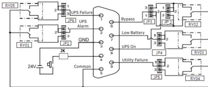
Fig 2 Connection for ACTIVE CLOSE
