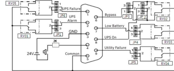
Fig. 3 Connection for ACTIVE OPEN
