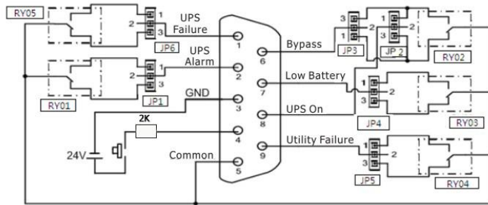
Fig 1 Pin definition and internal logical connection
