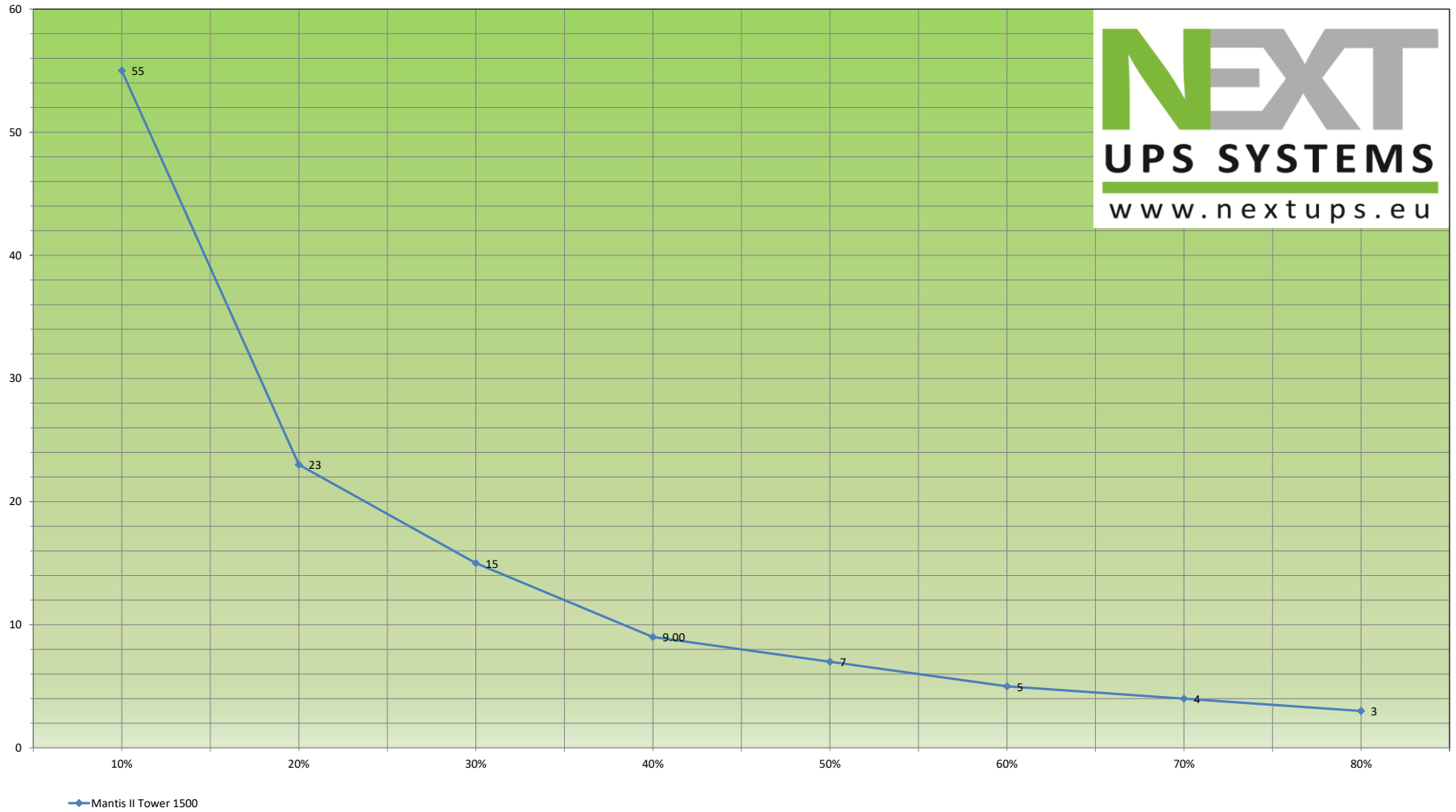
Mantis II 1500 with Pf=0,6 load (100% = 1500VA / 900W)
